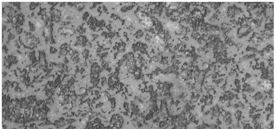
Micrograph showing the structure of SiC30 material under polarized light
