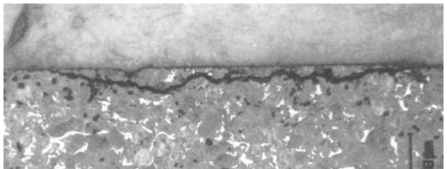
Typical appearance: Blistering on a carbon graphite seal
