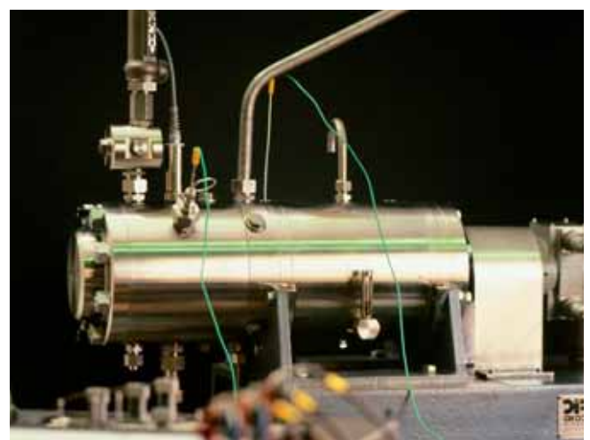
Evaluation rig for blister tests with high viscosity oil as sealed medium
