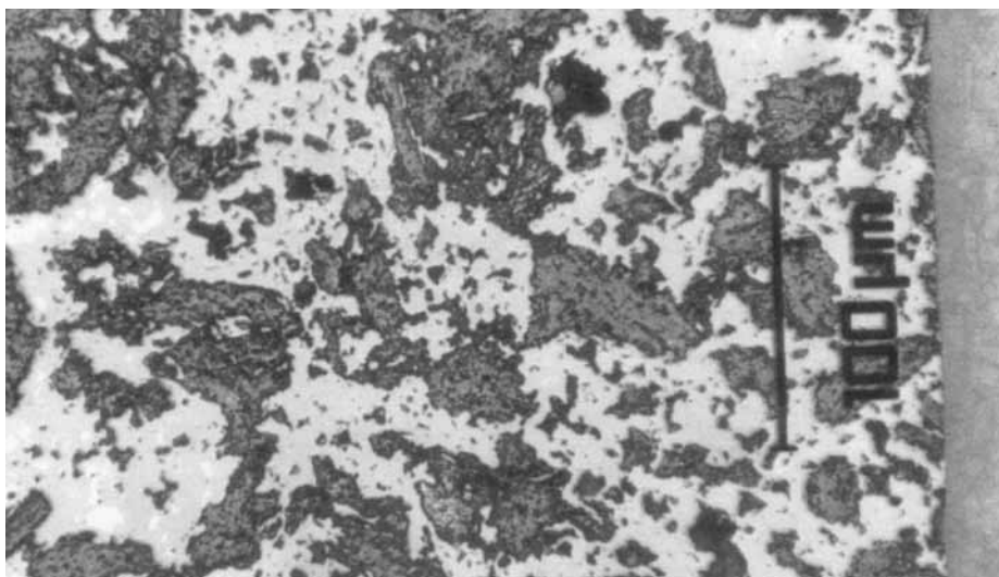
Micrograph of SiC30 after leaching in HF/HNO 3
